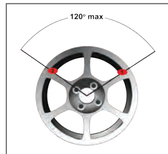
Split weight mode, adhesive weights can be hidden behind adjacent spokes of alloy rim
