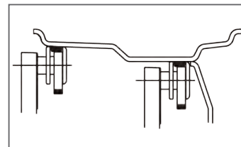
ALU 2P/3P mode for exact weight positioning
